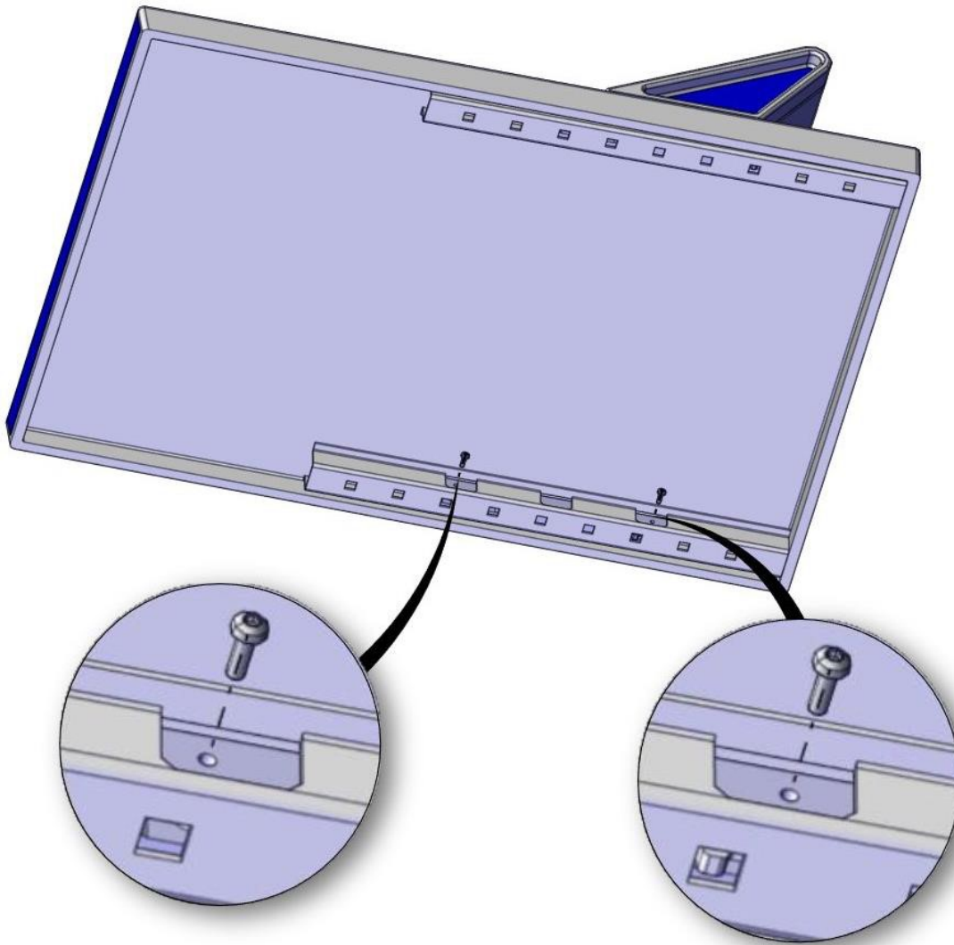
Figure 9 – Dismantling of the footrest
