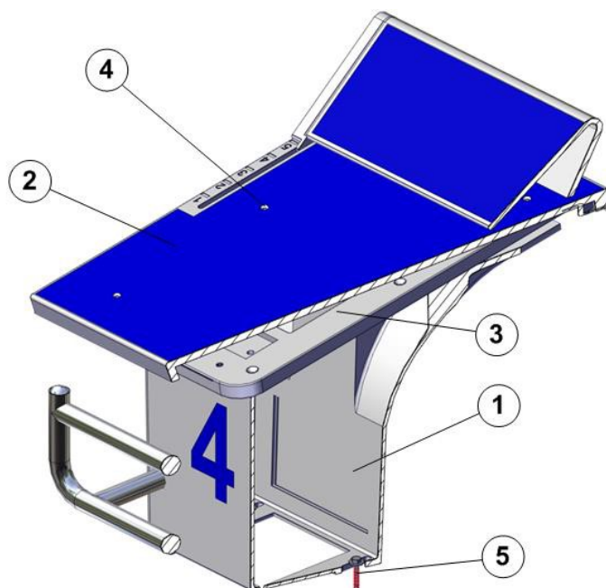
Figure 2 - OSB14 without RBD
