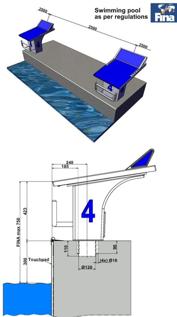
Figure 3 – Positioning of the OSB14
